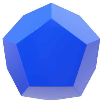
Dodecahedron
