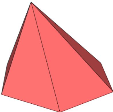
Hexagonal Pyramid
